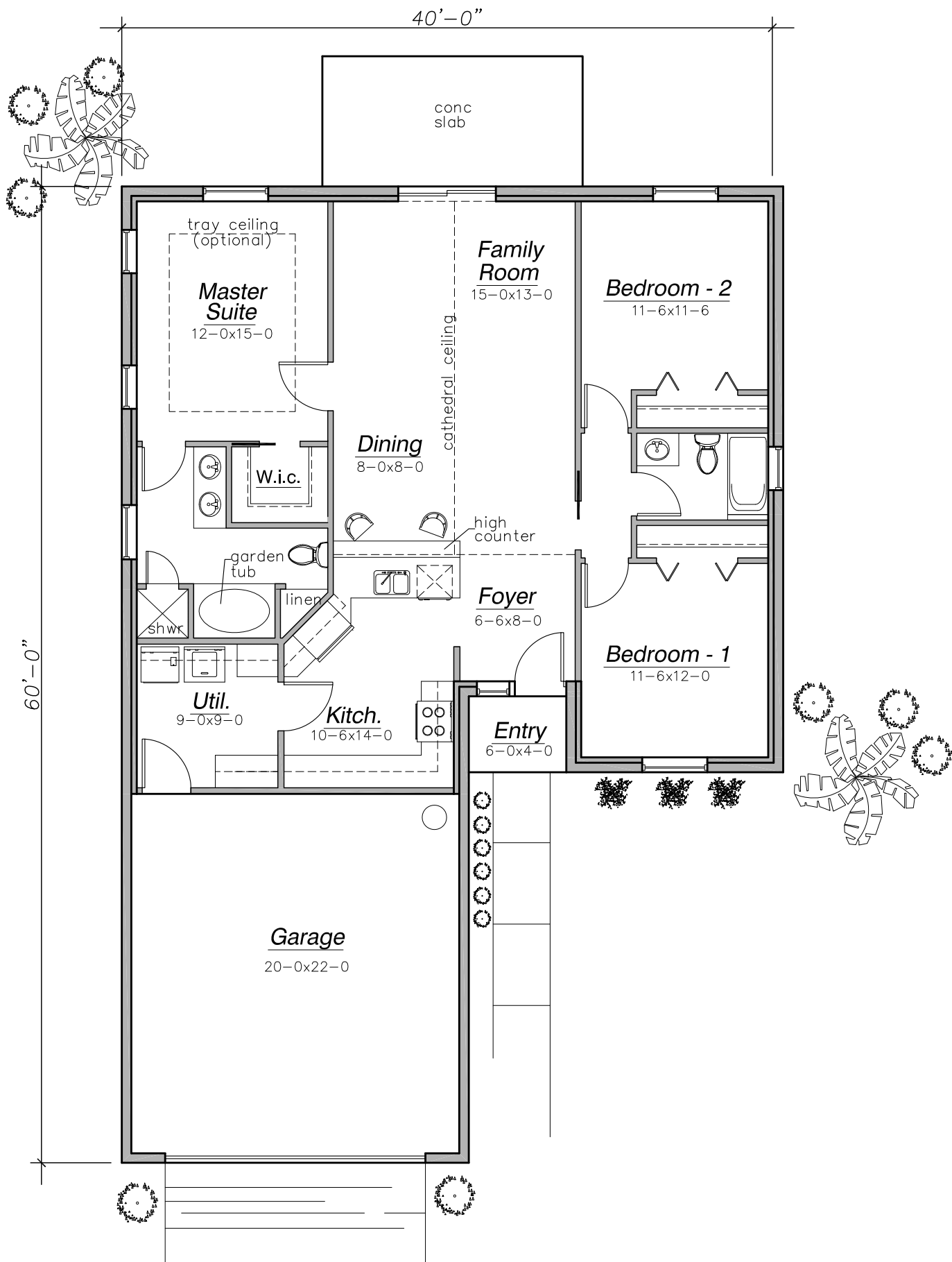
Optional Covered Lanai 160 s.f. of Lanai Area
